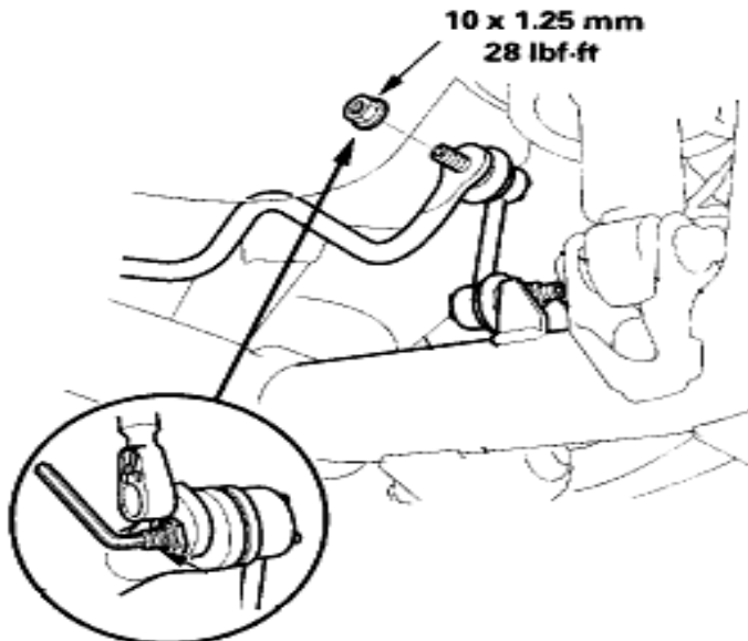
(Illustration 7) Rear factory end link
