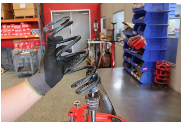
Step 9. Remove the OE secondary spring.
