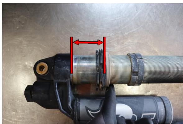
Step 10. Set pre-load of spring seat to 95mm (3 3/4in.) from the bottom of the seat to bottom of the reservoir bridge.
