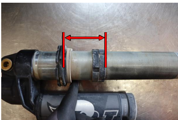
Step 11. Set the crossover ring to 85mm (3 3/8in.) from the bottom of the spring seat to the bottom of the crossover ring.
