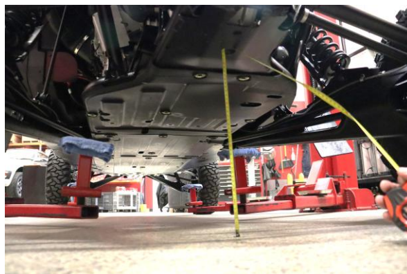
Step 22. Lower the vehicle and carefully test drive while listening for any abnormal noises. Measure from the ground to the center of the skid plate between the rear mount of the front lower control arms. The recommended preload measurement in Step 13 will get the vehicle close to the recommended ride height but each vehicle may vary some. We recommend setting the ride height at 485mm (16.75in.) measuring from the ground to the center of the front skid plate/ ground clearance. Note: Measurements were taken from a vehicle with 32in. tires. If your vehicle has a different size tire, the ride height will need to be adjusted. Due to the sensitivity of weight of these vehicles, weight distribution may change ride heights, additional pre-load may need to be added to compensate.
