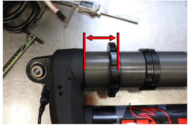
Step 14. Set pre-load of spring seat to 70mm (2 3/4 in.) from bottom of seat to bottom of reservoir bridge.
