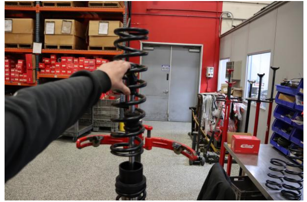
Step 8. Decompress the spring assembly. Remove the OE rear main spring.
