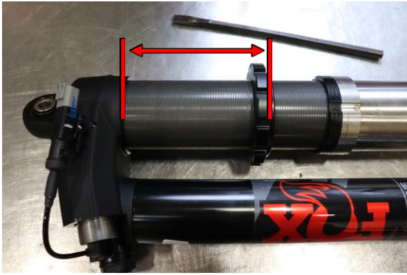
Step 13. Set pre-load of spring seat to 145mm (5 11/16in.) from bottom of seat to bottom of reservoir bridge.
