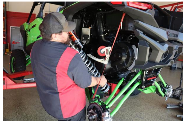
Step 18. Install the shock in the vehicle.
