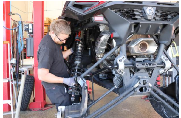
Step 6. Remove shock from car.
