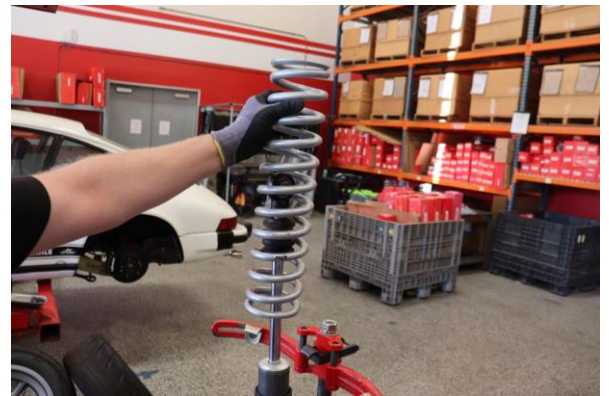
Step 18. Install Eibach front main spring.
