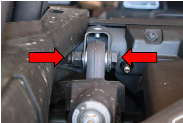
Step 3. Remove 21mm upper shock mount nut and bolt with 21mm socket and wrench.
