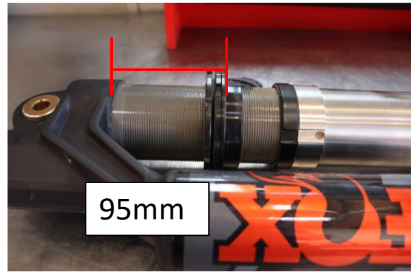
Step 14. Set pre-load spring seat to 95mm (3 47/64in.) from bottom of seat to bottom of reservoir bridge.
