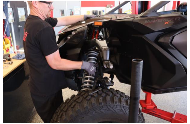
Step 20. Install shock in vehicle using upper mount bolt to hold assembly in place.
