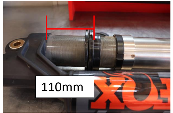
Step 14. Set pre-load spring seat to 110mm (4 11/32in.) from bottom of seat to bottom of reservoir bridge.
