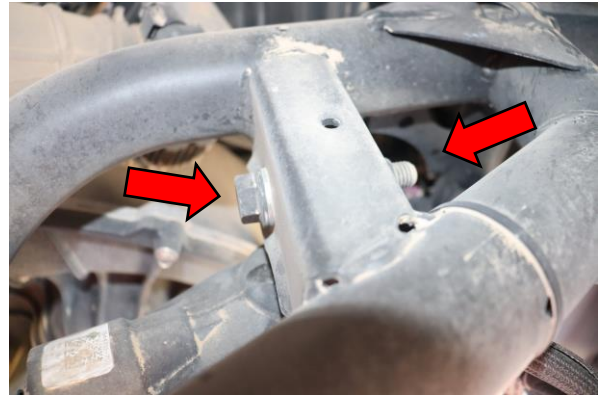
Step 20. Use two 18mm to install upper shock mount nut and bolt. Tighten to factory specification.
