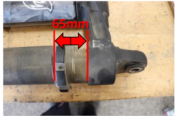
Step 14. Remove shock from the spring compressor. Adjust the upper spring perch to 65mm (2 9/16in) measuring from the spring seat to the bottom of the bridge to set spring preload.
