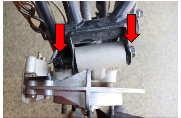
Step 22. Use two 21mm to install the upper control arm to hub nut and bolt. Tighten to factory specification.
