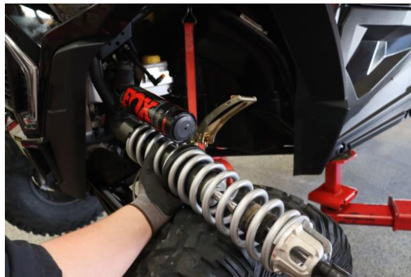
Step 18. Place the shock assembly in the vehicle and begin to mount using the upper shock mounting bolt. Lift slightly on the tire and install the lower shock mounting bolt.
