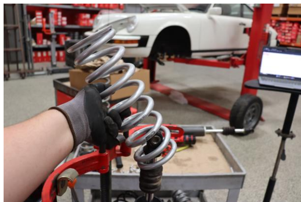
Step 16. Install the Eibach main spring.
