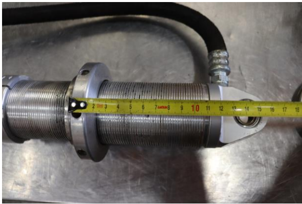
Step 13. Set pre-load to 115mm (4 1/2") from bottom of spring seat to bottom of reservoir bridge collar.
