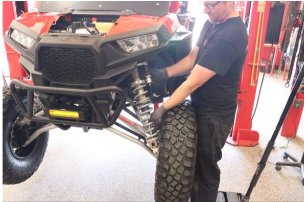
Step 16. Install shock assembly in the vehicle
