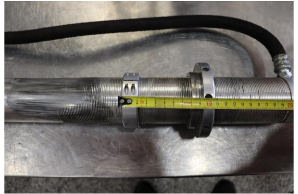
Step 14. Adjust the Eibach supplied crossover ring to 95mm (3 ¾") from bottom of spring seat to bottom of crossover ring.
