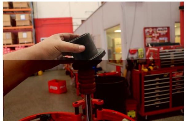
Step 18. Install Eibach spring slider with the short end facing the top of the shock.
