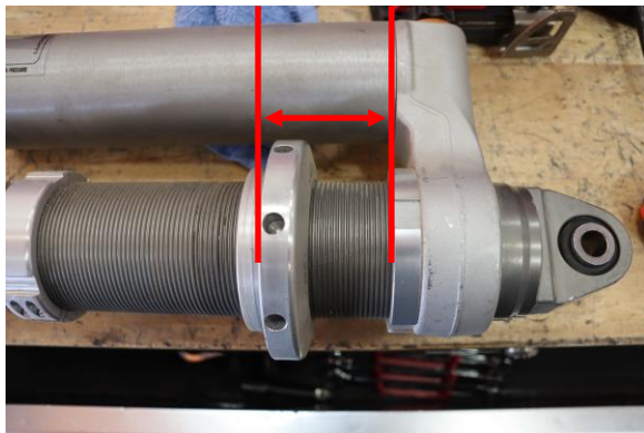
Step 15. Set pre-load to 55mm (2 5/32in.) from bottom of spring seat to bottom of reservoir bridge collar.
