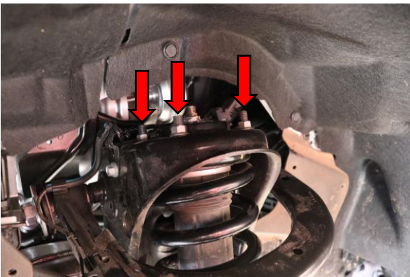
Step 11. Remove the four 14mm top hat nuts securing shock assembly to the frame.
