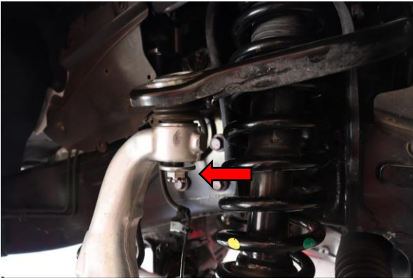
Step 7. Loosen, but do not remove the 19mm nut securing the spindle to the upper control arm.
