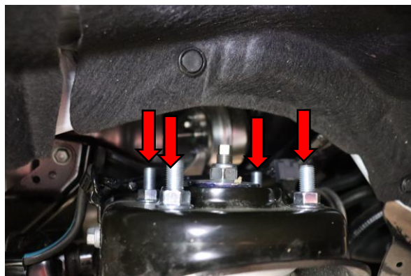
Step 17. Use a 14mm wrench to tighten four upper shock mounting nuts to factory specification.
