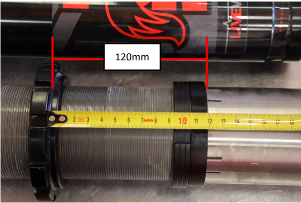
Set the crossover rings to 120mm from the spring seat to the bottom of the crossover rings.
