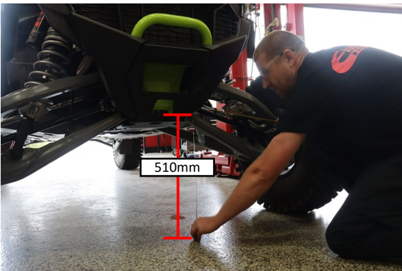
The front ride height should be about 510mm front the ground to the lower control arm bolt.
