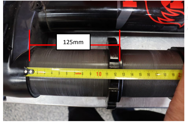
Set the rear preload to 125mm from the bottom of the Resi bridge to the spring seat.
