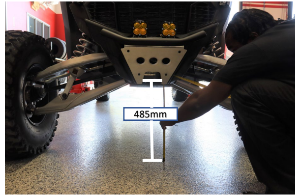
The front height should measure about 485mm from the ground to the lower control arm bolt. The shock eye to eye length should be about 785mm.
