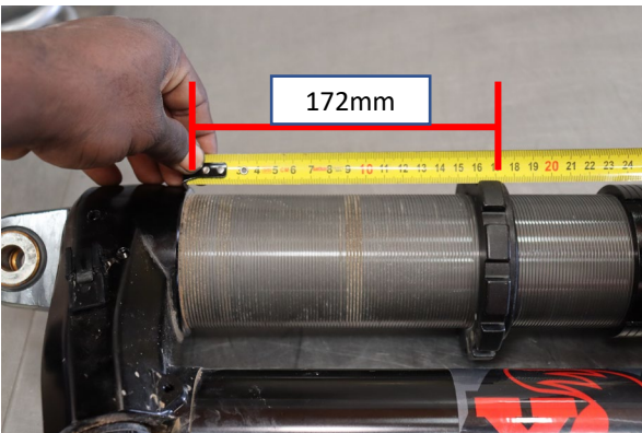
Set the preload collar to 172mm from the bottom of the resi bridge to the bottom of the spring perch
