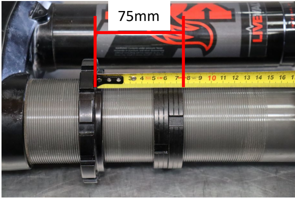
Set the OE crossover ring to 75mm
