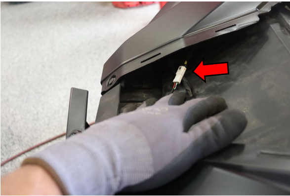
The front camera is attached to this assembly. Unplug and set aside.
