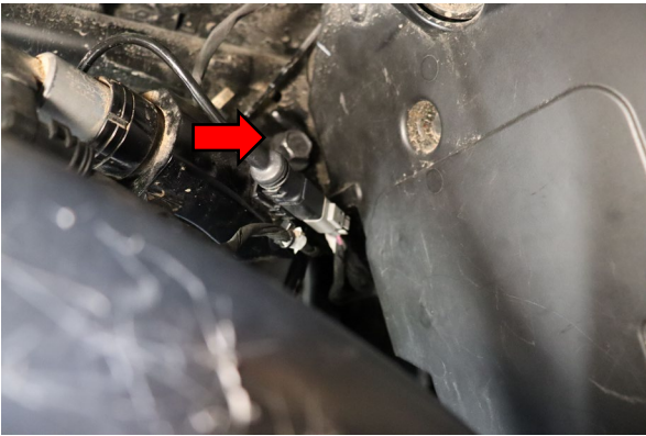
Remove the upper shock bolt with a 21mm socket.
