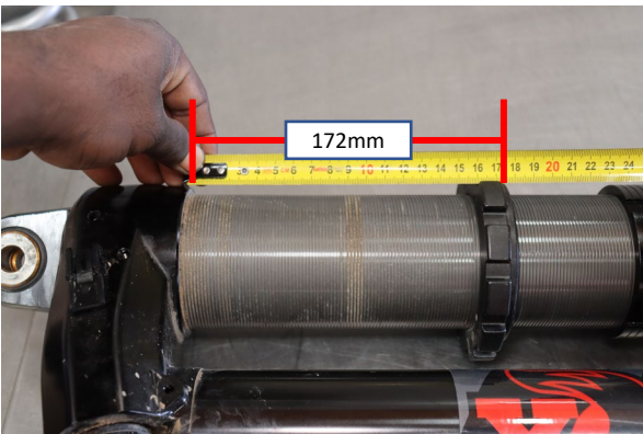
Set the preload collar to 172mm from the bottom of the resi bridge to the bottom of the preload collar.
