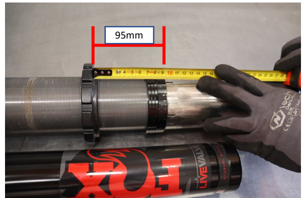
Set the crossover ring to 95mm. From the bottom of the spring collar to the bottom of the crossover ring.
