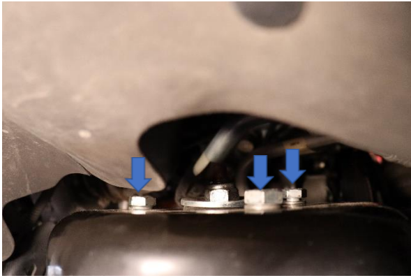
Step 12. Install the 3 14mm nuts provided with the kit to secure the top hat to the shock tower.
